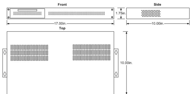
Chassis Mechanical Drawing
